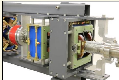
AC Scanning Magnet
