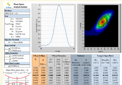
Phase Space Analysis Software
