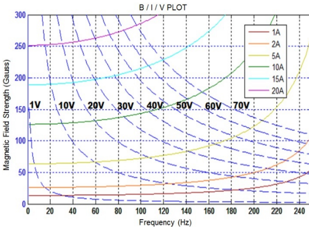
Figure 5: Magnetic field as a function of frequency for power supply sinusoidal peak current values up to \pm 20 Amps and, for the case of the KEPKO BOP 50-20 GL power supply, a maximum of \pm 50 Volts.
