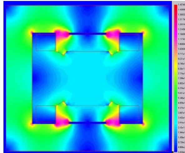
Figure 2: Magnetic field in Tesla. Each Rose shim is a triangle with base 20 mm in horizontal plane and height 8 mm at a point \frac{3}{4} along the base. Each Purcell filter is an absence of C1010 material, centred at the pole base, 4 mm in height by 72 mm in width.
