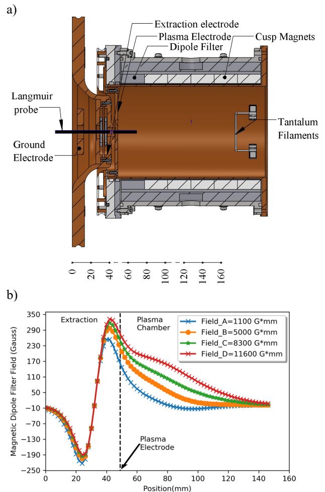
Figure 1: a) Schematic of the filament based multicusp ion source. b) Different magnetic dipole filter fields used for this study. The magnitude of field indicated is the integrated field over length in the plasma chamber.
