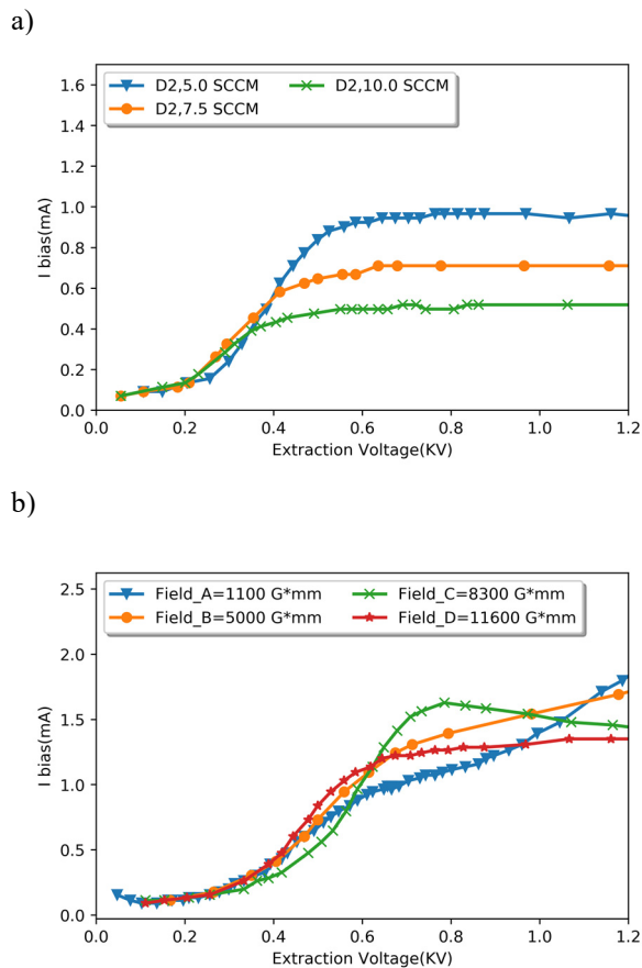
Figure 4: a) Variation of I_{bias} for different gas flows at a constant arc current of 5.0 A for Field_D. b) Variation of I_{bias} for different magnetic dipole strengths at arc current of 6.5 A and arc voltage of 120.0V.
